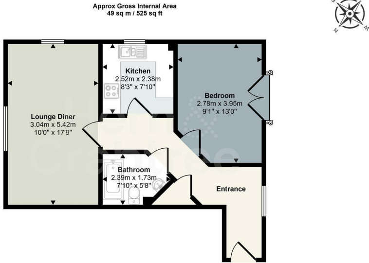
Floorplan
